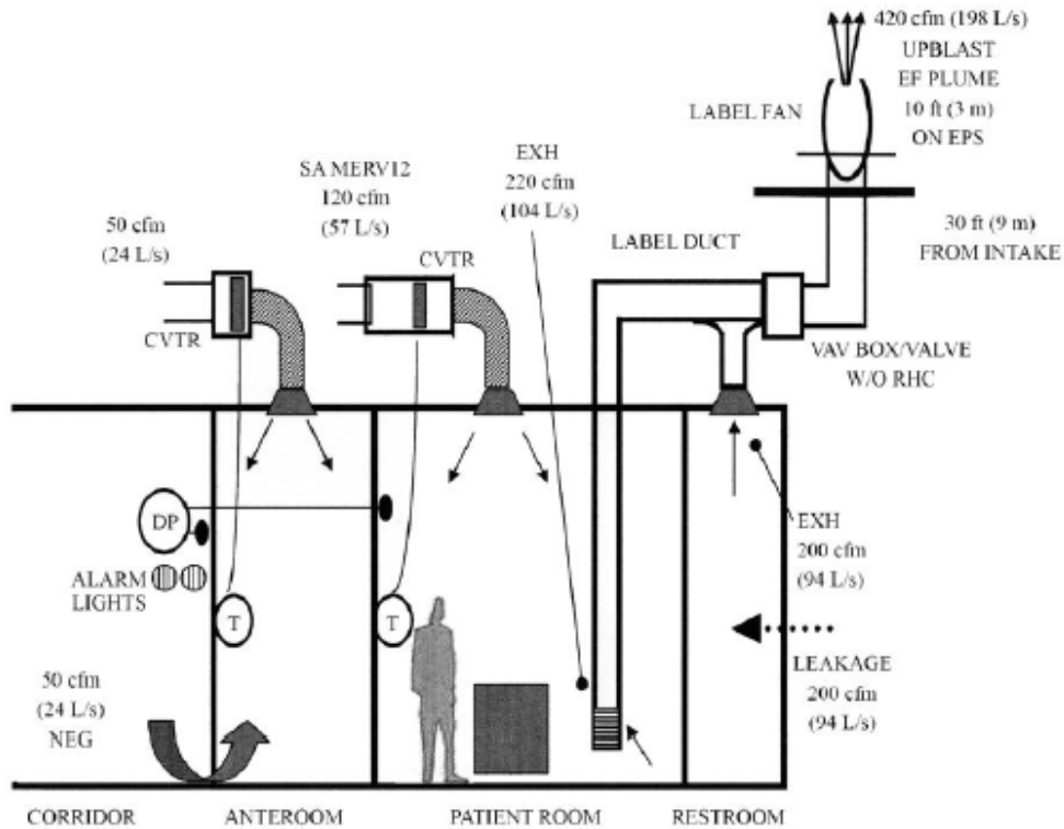
Figure 8-17 Airborne Infectious Isolation (AII) Room Arrangement
